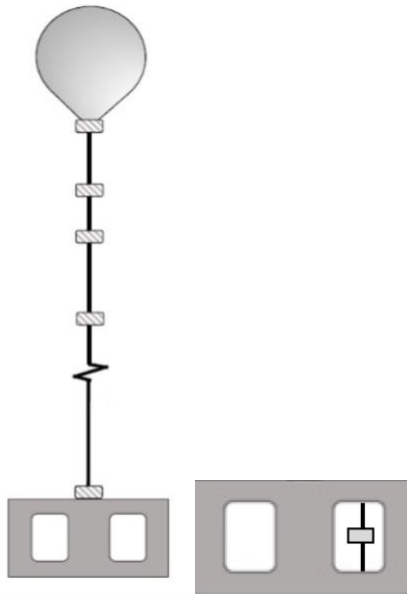
Figure 5. Illustration of the temperature sensor arrays deployed at Bloody Creek and Belleisle Marsh (left), and the single temperature sensors deployed in Paradise, Daniels Brook, and Bridgetown (right).
