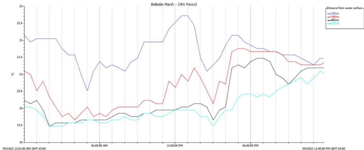
Figure 14. Data from Belleisle Marsh showing the temperature at varying depths on September 24 th .
